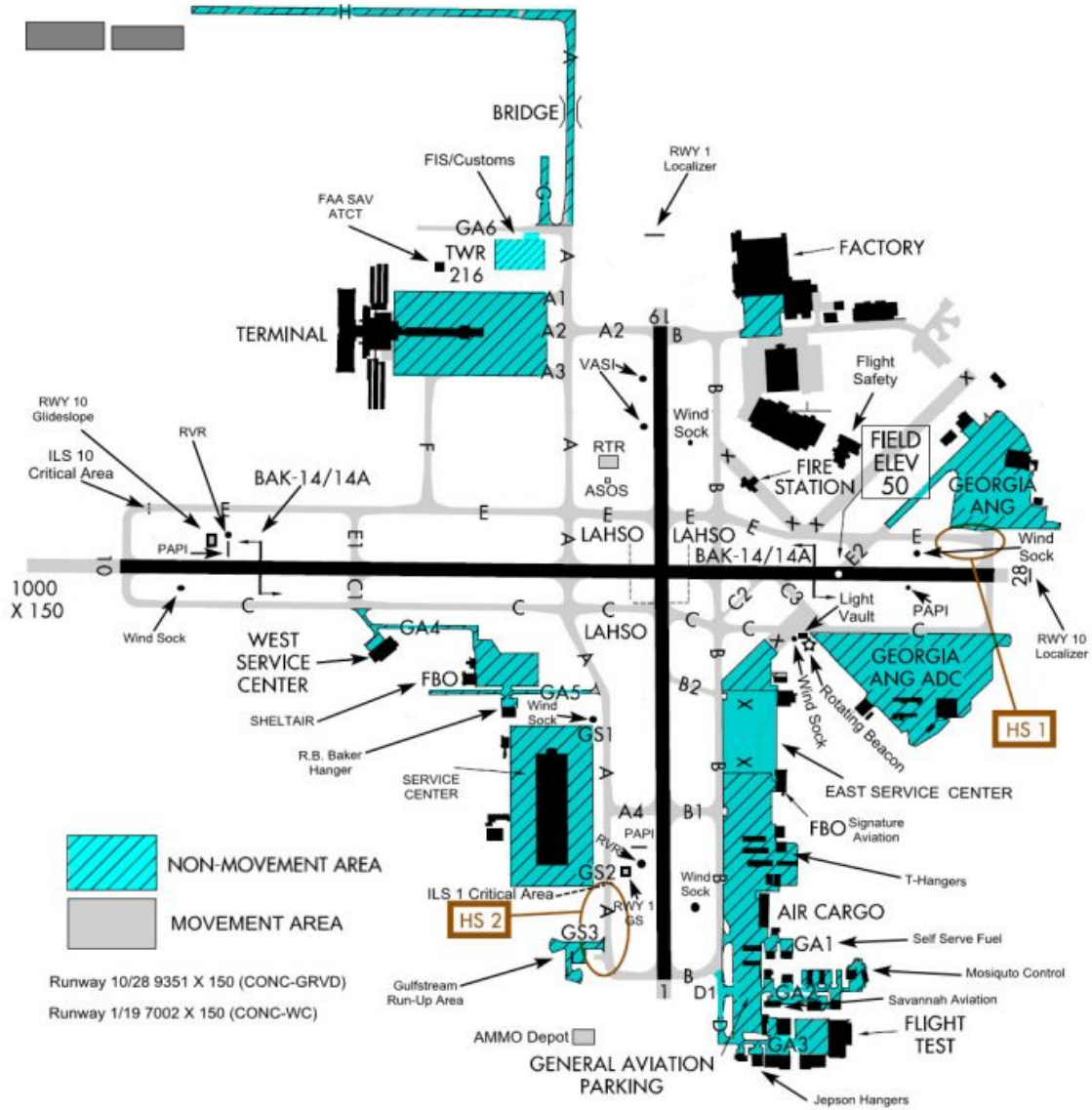
Figure 1. Ground Movement and Non-Movement Areas
