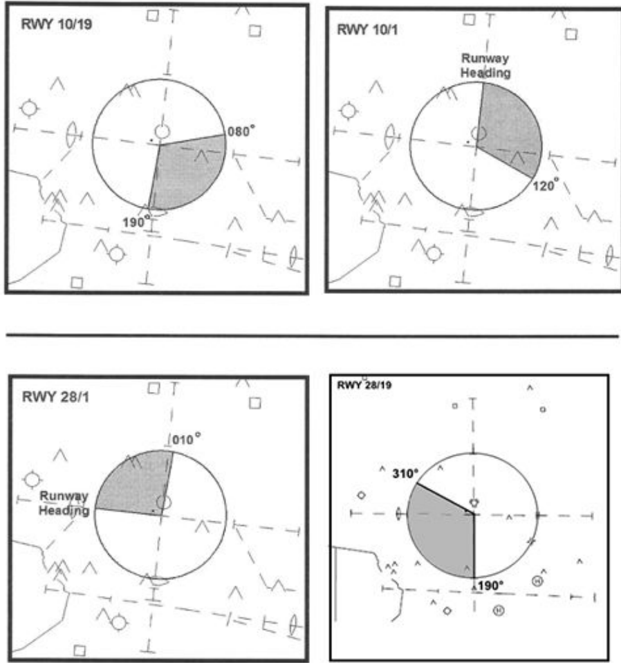
Figure 3. Departure Headings
