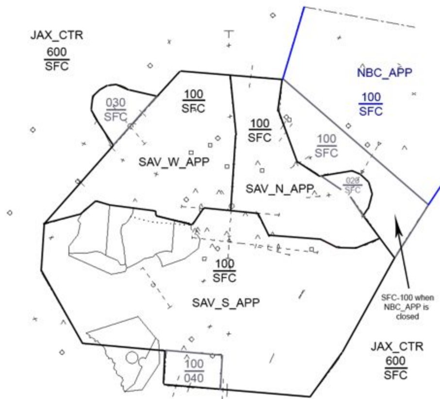
Figure 5. SAV TRACON and Adjoining Airspaces
