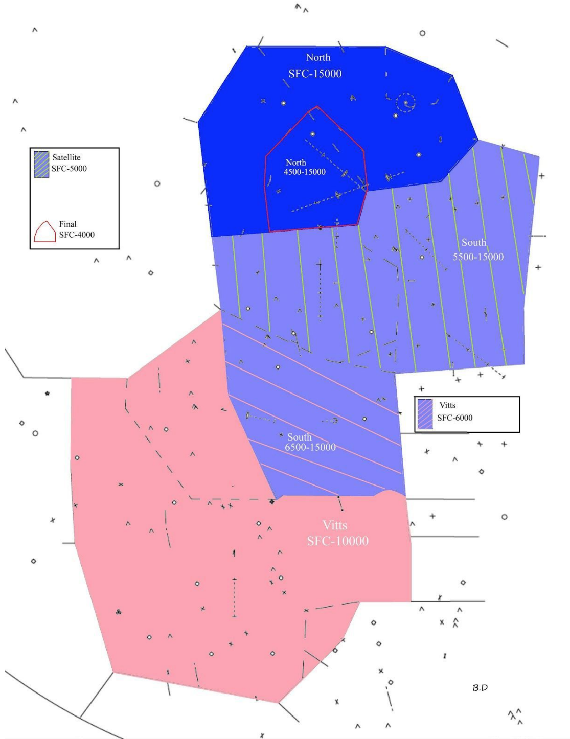
Figure 3. Jacksonville TRACON, East Operations
