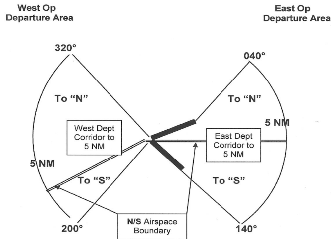
Figure 1. Piston Standard Departure Headings
